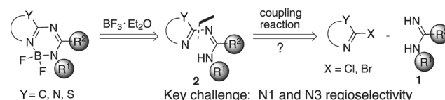
Scheme 1. Design of a target-directed coupling reaction for the proposed N_3C_2/BF_2 dyes.
